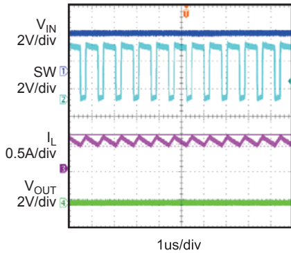
Short Circuit Steady Waveform
